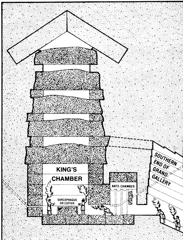
Vertical Section (looking west) of KING'S CHAMBER; also of ANTE-CHAMBER, South End of GRAND GALLERY and Vyse's Hollows of Construction above King's Chamber.
